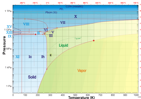
Figure 2. T - P Phase diagram for water, taken from http://www1.lsbu.ac.uk/water/phase.html .
