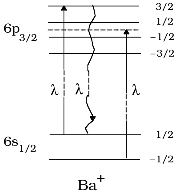
Fig. 4. Relevant energy spectrum of the valence electron of Ba^+ immersed in a magnetic field. The jump in energy from the 6s_{1/2} to the 6p_{3/2} levels is several orders of magnitude greater than it appears in the sketch. Laser-induced fluorescence (LIF) can occur when an electron in the upper 6s_{1/2} level can absorb a photon of wavelength \lambda , jump to the highest 6p_{3/2} level, then re-emit the photon and return to the upper 6s_{1/2} level. If the electron is initially in the lower 6s_{1/2} level, then absorbing the same photon of wavelength \lambda can excite it only as high as the dotted line in the middle of the 6p_{3/2} multiplet, where no level exists. Then LIF cannot occur. Data taken from Moore 10 .
