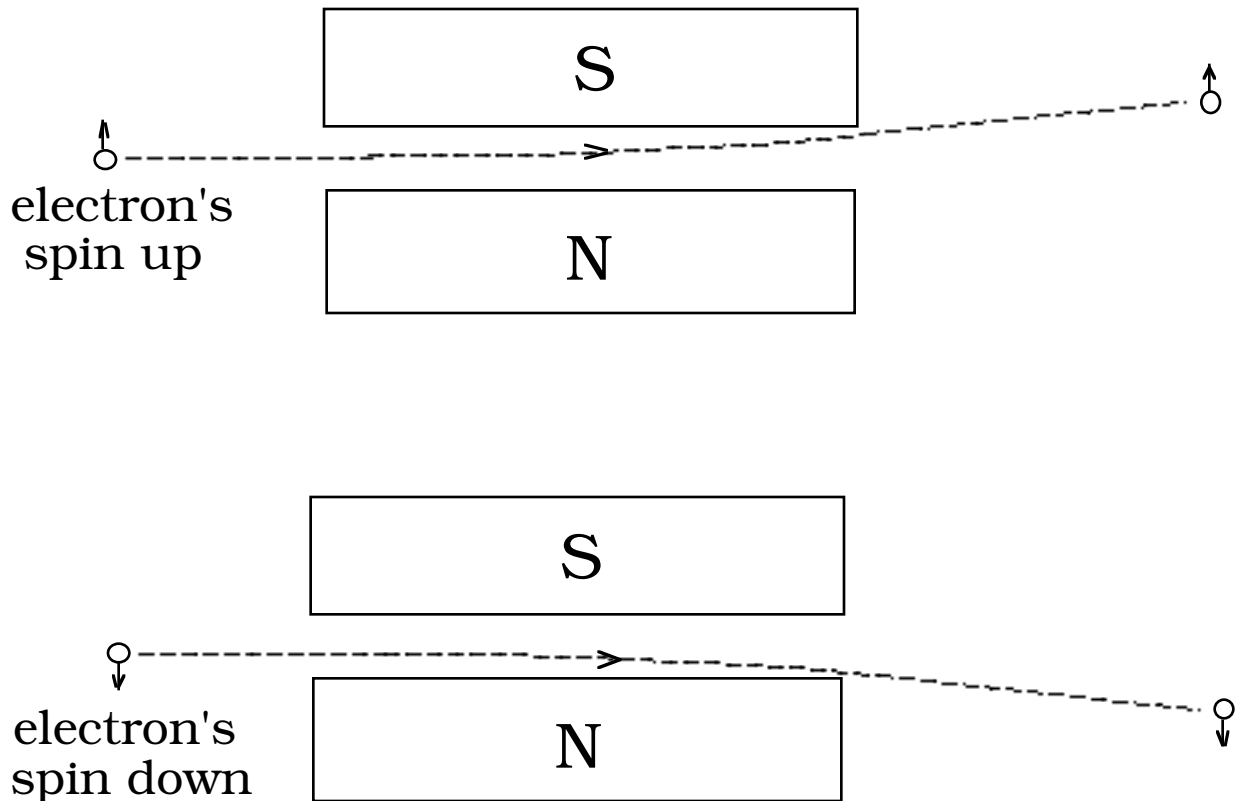
Fig. 2. Highly divergent magnetic field between poles of a Stern-Gerlach device causing electron with spin “up” to be deflected upward, and electron with spin “down” to be deflected downward.
