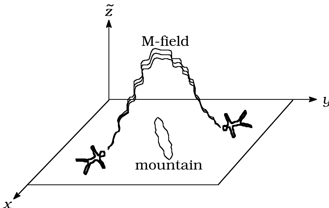
Fig. 5. To visualize an extra dimension, imagine that we live in just a two-dimensional x, y plane, as in Abbott's Flatland 20 . The extra dimension rises vertically from our plane and is denoted z -twiddle ( \tilde{z} ). We can't see in that
