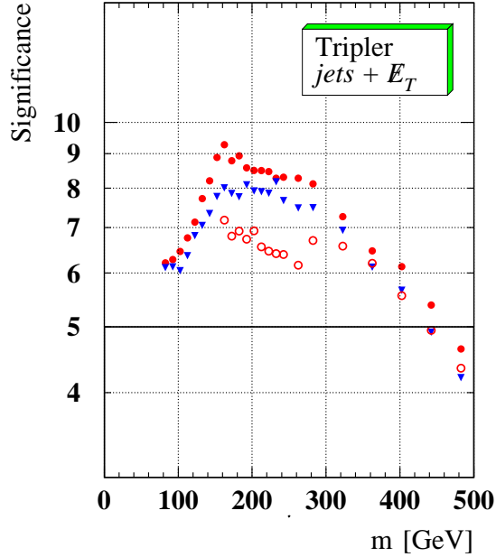
FIG. 3. Significance as a function of m_0 at m_{1/2} = 410 GeV ( m_{\tilde{g}} \simeq 980 GeV) for \tan \beta = 3 (filled circles), 10 (down triangles), and 30 (open circles) in jets + \cancel{E}_T channel at the Tripler. m_0 \lesssim 150 GeV is theoretically forbidden for \tan \beta = 30 .
